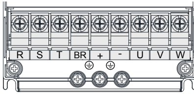
Figure 3-9 Terminal arrangement in MD500T0.4GB to MD500T15GB and MD500-2T0.4GB to MD500-2T7.5GB
