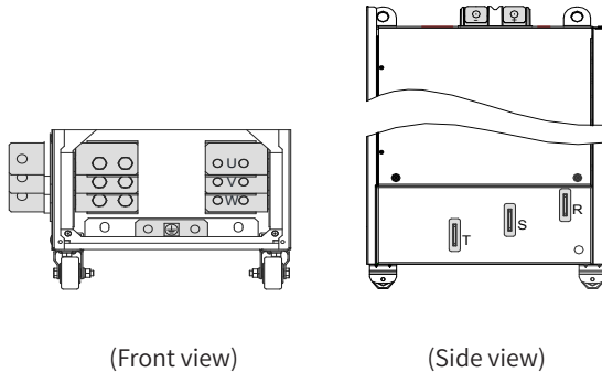
Figure 3-11 Terminal arrangement in MD500T200G(-L) to MD500T450G(-L)
